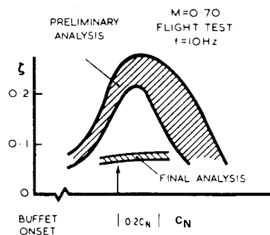
Fig. 1 Apparent damping of first wing-bending mode (Ref. 1).
